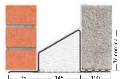
150-165mm cavity
