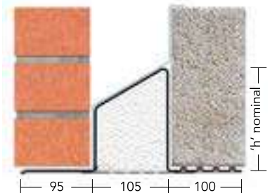
110-125mm cavity
