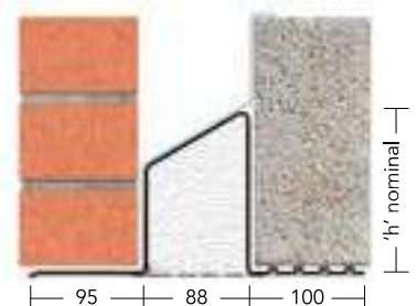
90-105mm cavity
